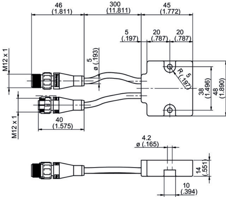
2x cable with connector M12
