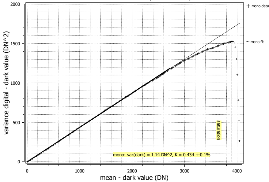
Photon transfer mACC300044, 533 nm, 14.03.2023
