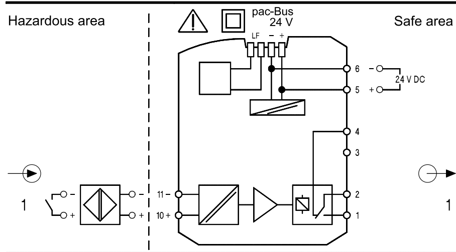
Connection diagram
