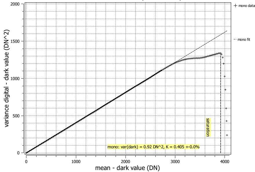
Photon transfer mACC300034, 533 nm, 09.03.2023
