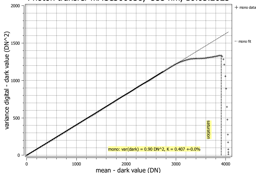
Photon transfer mACC300038, 533 nm, 10.03.2023
