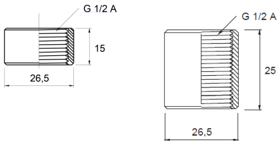
ZPW1-723 G 1/2 A (Fitting BCID: G06, G44, G51)
