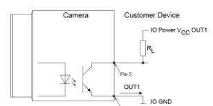
Digital Output: Low Active
