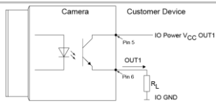
Digital Output: High Active
