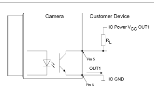
Digital Output: Low Active
