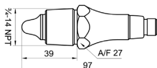
LBFS-xx6xx.x 3/4-14 NPT (BCID: N03)
