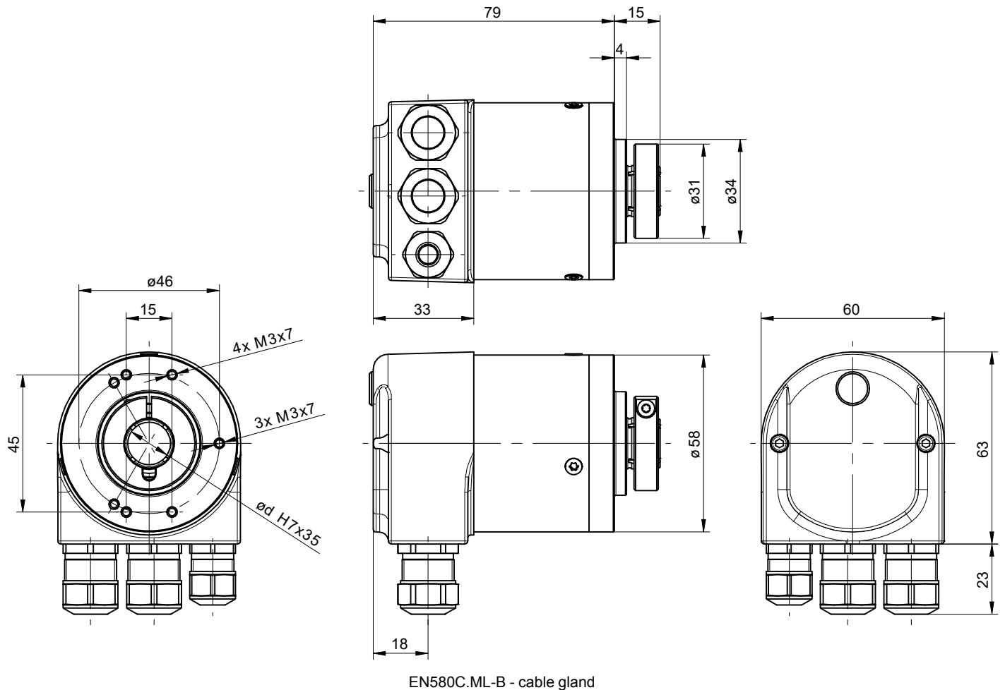
EN580C.ML-B - cable gland
