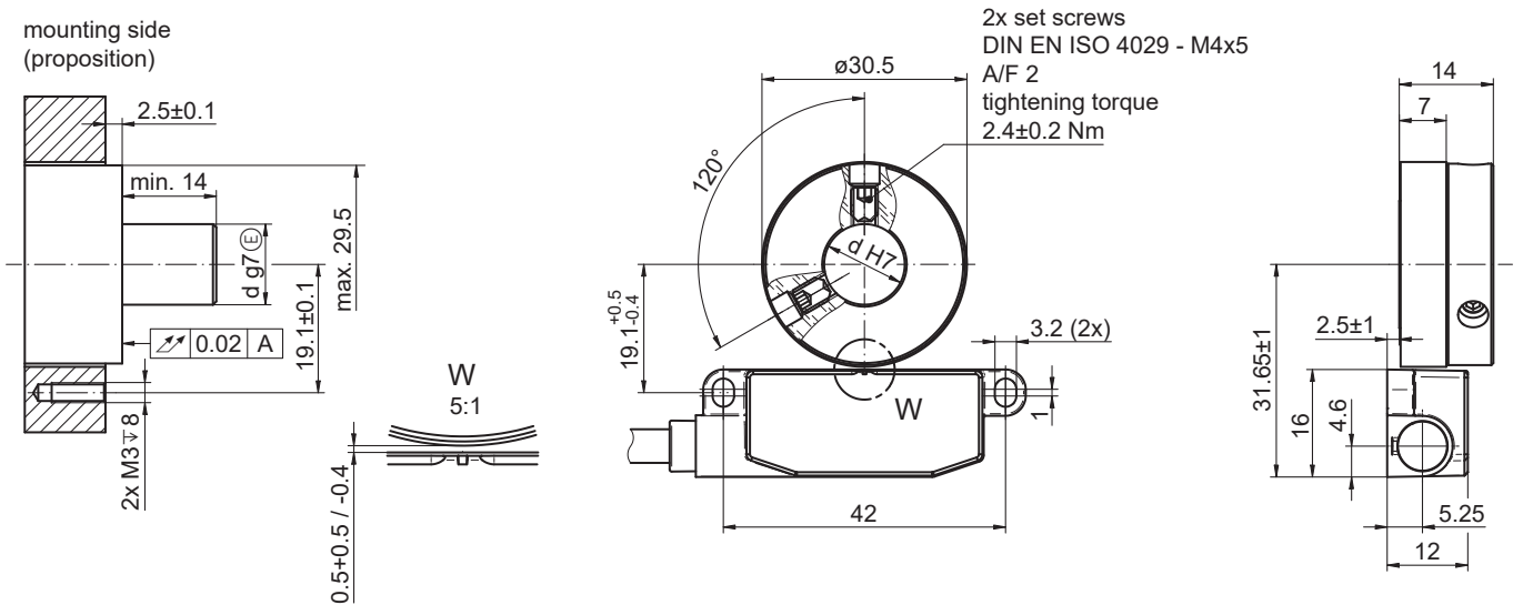
EB200E.IR-FN with EBS.R-FN032.S for screw mounting
