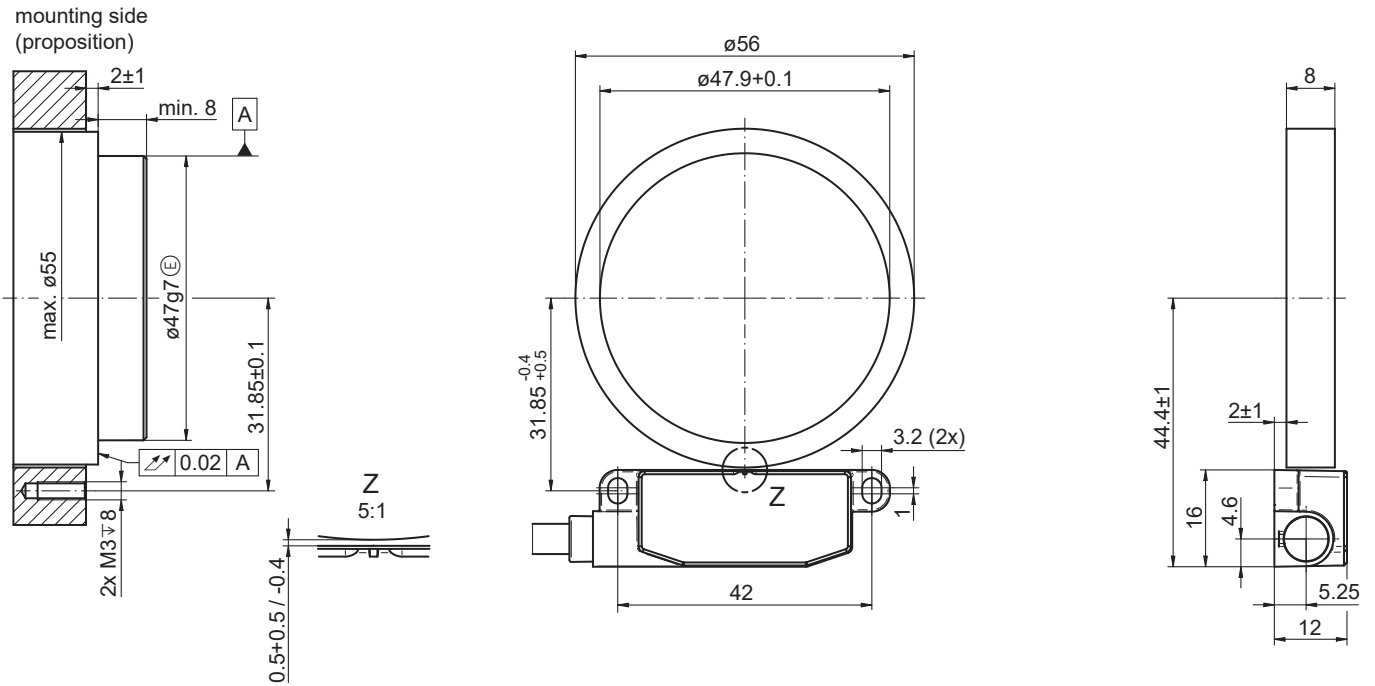
EB200E.IR-FN with EBS.R-FN032.B for bonding
