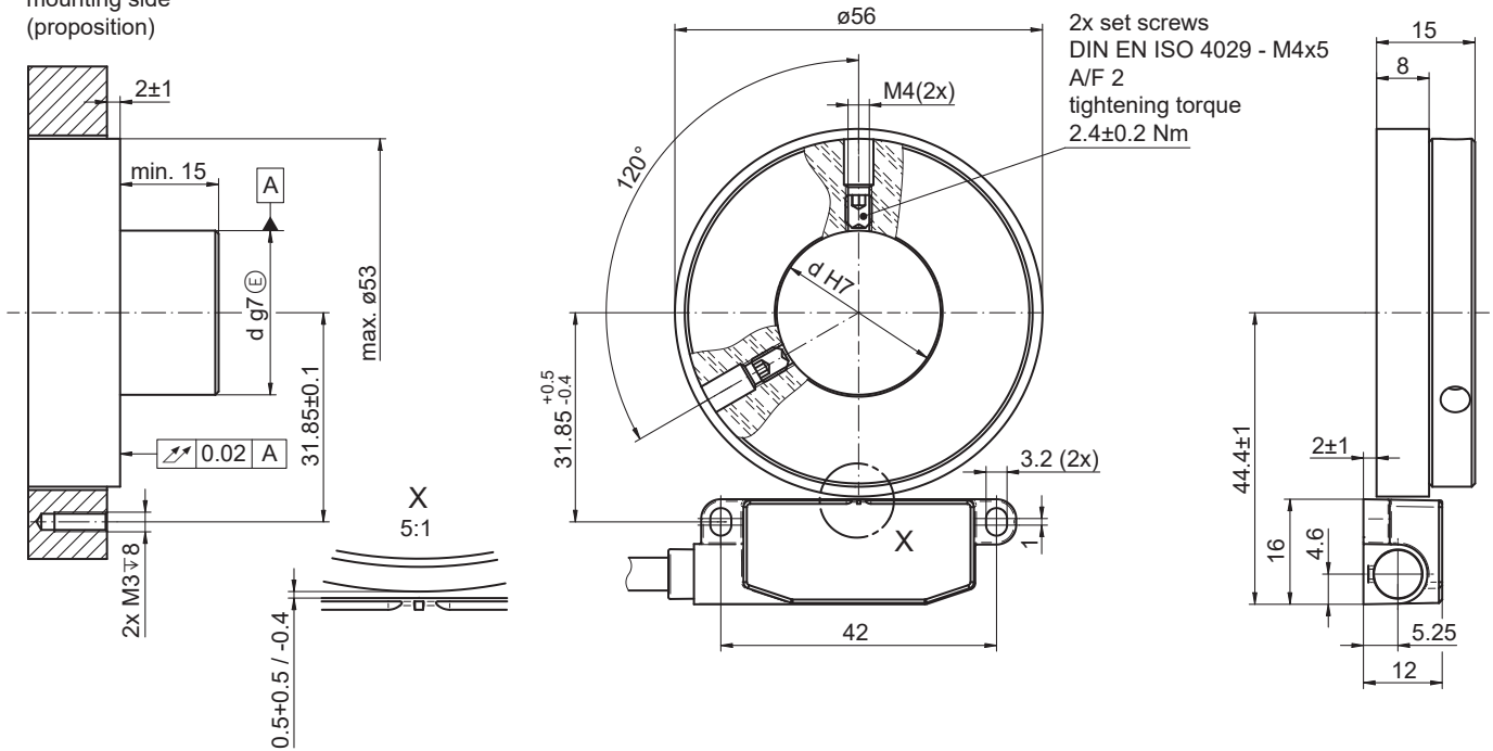
EB200E.IR-FN with EBS.R-FN064.S for screw mounting
