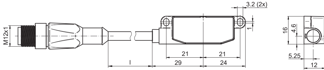
EB200E.IR-FN with cable and connector M12
