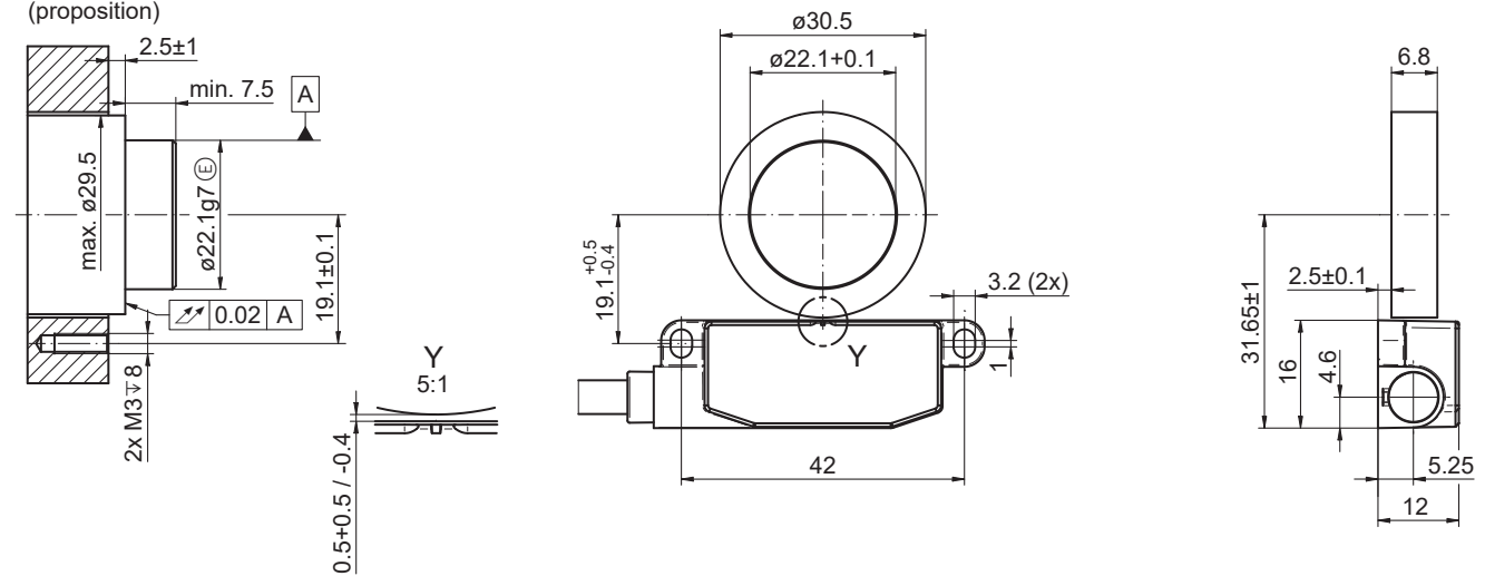
EB200E.IR-FN with EBS.R-FN032.B for bonding
